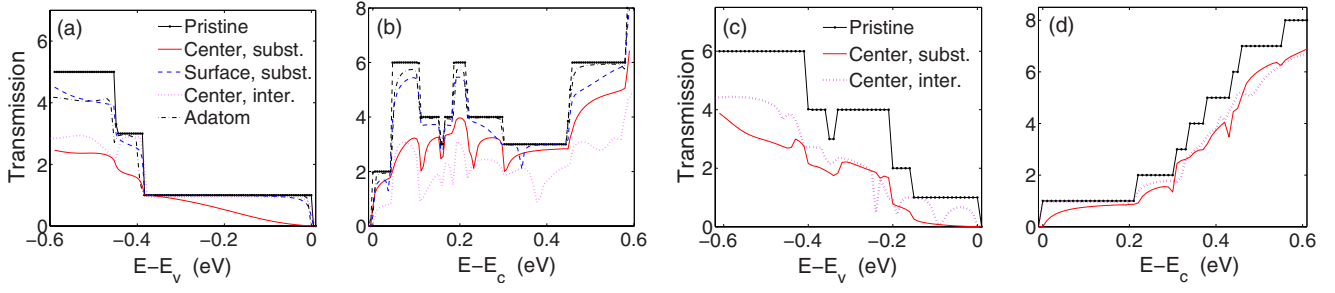
FIG. 5. (Color online) Transmission through D=16 Å \langle 111 \rangle SiNWs (a)-(b) with the Au atom in different positions: Substitutional in the center of the wire (solid), substitutional at the surface (dashed), interstitial in the center (small dotted), surface adatom (dash dotted). The pristine wire transmission is indicated by larger dots. Panels (c) and (d) show transmission through the D=12 Å \langle 110 \rangle SiNW with the Au in a substitutional and interstitial position in the center of the wire.
