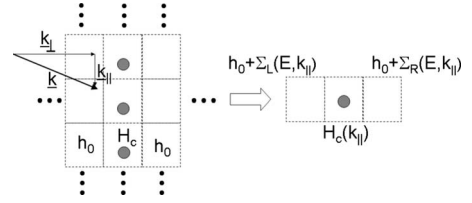
FIG. 2. Schematic 2D drawing of the bulk scattering method. k_\perp denote the transport direction, and the transmission is k_\parallel point sampled over k_\parallel .
